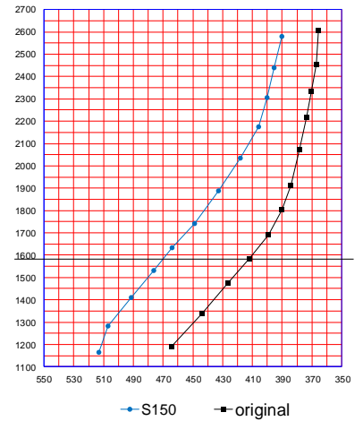
Spring characteristic Front Springs
